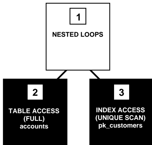
Figure 23-2 Execution Plan for a Nested Loops Join
