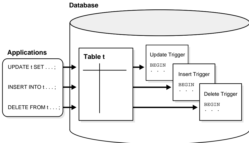
Figure 20–1 Triggers
