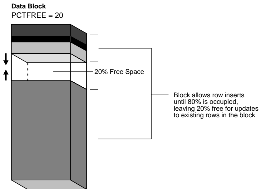
Figure 4-3 PCTFREE
