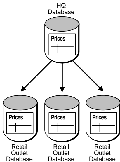
Figure 34–9 Information Distribution
