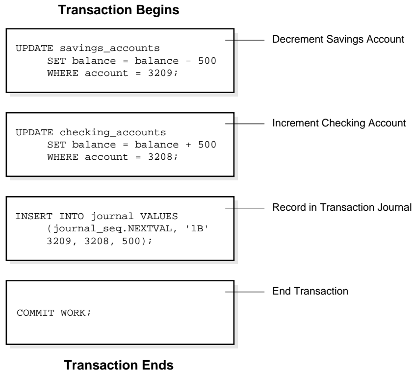
Figure 17-1 A Banking Transaction
