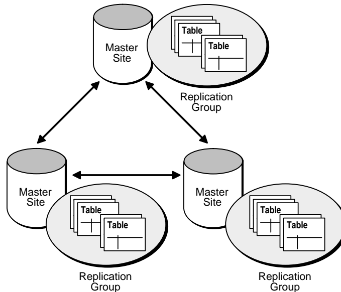
Figure 34-4 Multimaster Replication System
