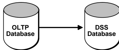
Figure 34–8 Information Off-Loading
