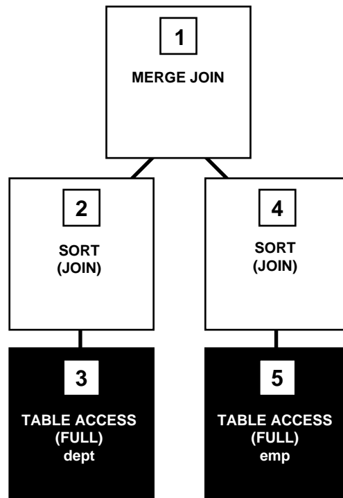
Figure 24–2 Sort-Merge Join
