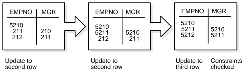
Figure 28–9 Constraint Checking
