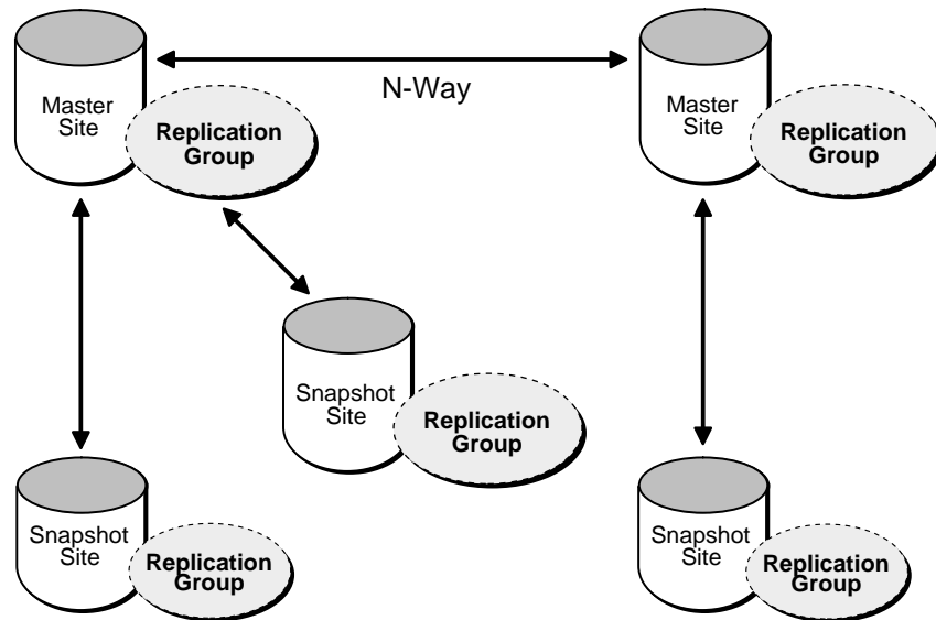
Figure 34-10 Hybrid Configuration
