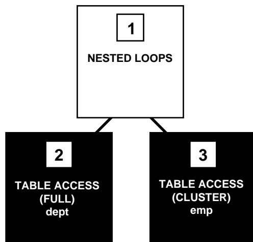
Figure 24–3 Cluster Join
