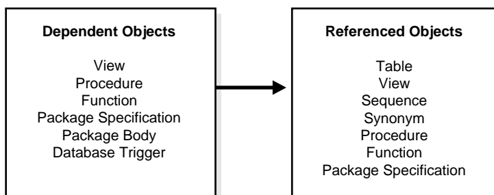
Figure 21-1 Types of Possible Dependent and Referenced Schema Objects
