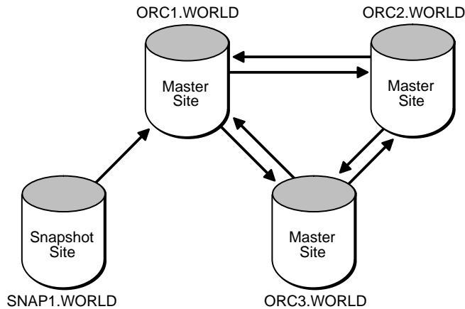
Figure 34–3 Three Master Sites and One Snapshot Site
