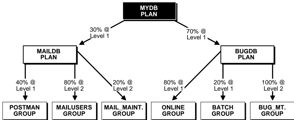
Figure 9–1 Subplans: Resource Plans That Refer to Each Other
