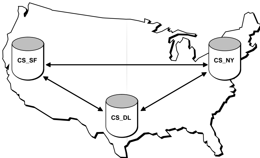
Figure 34–5 Multimaster Replication Supporting Multiple Points of Update Access
