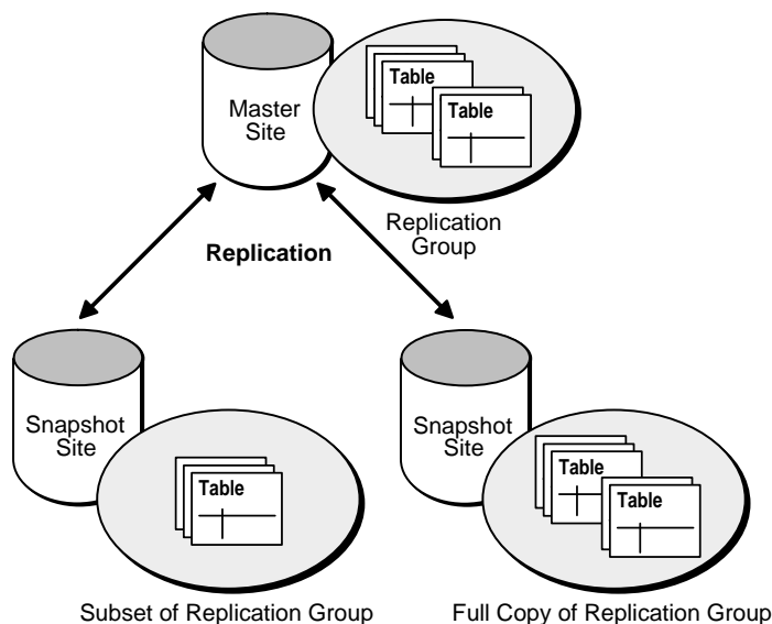
Figure 34–7 Updateable Snapshot Replication
