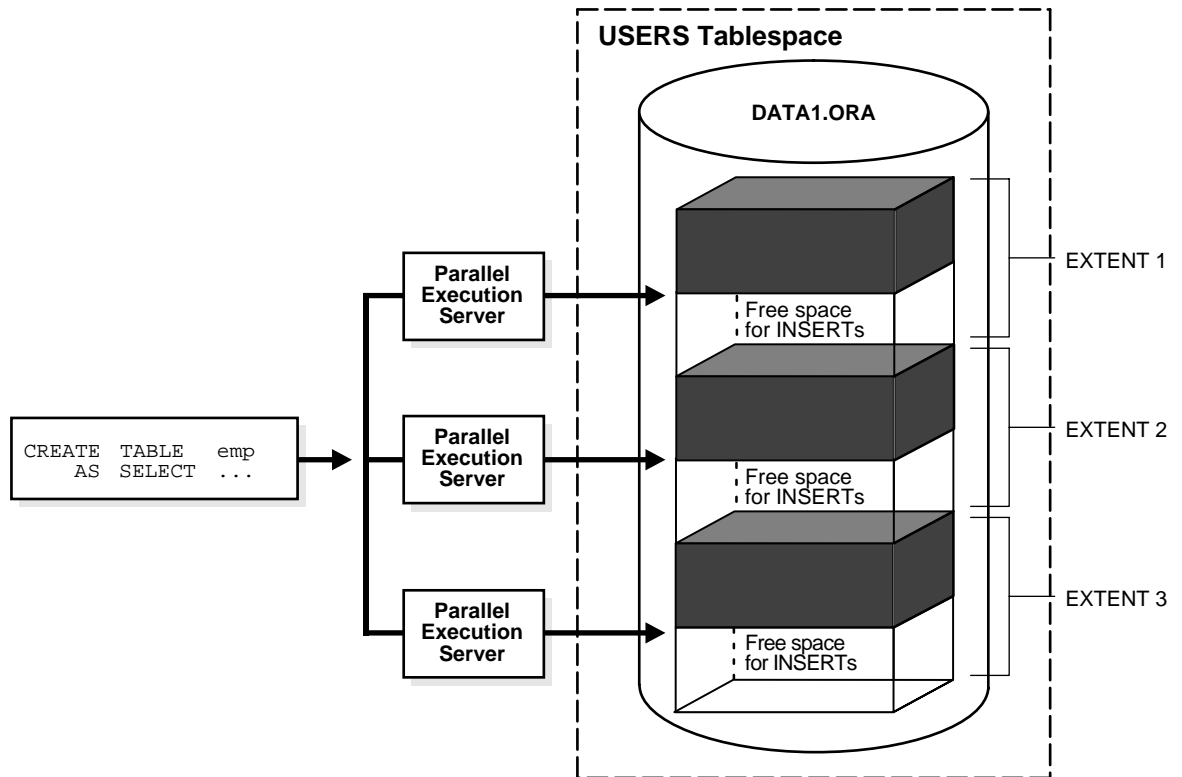
Figure 26–7 Unusable Free Space (Internal Fragmentation)
