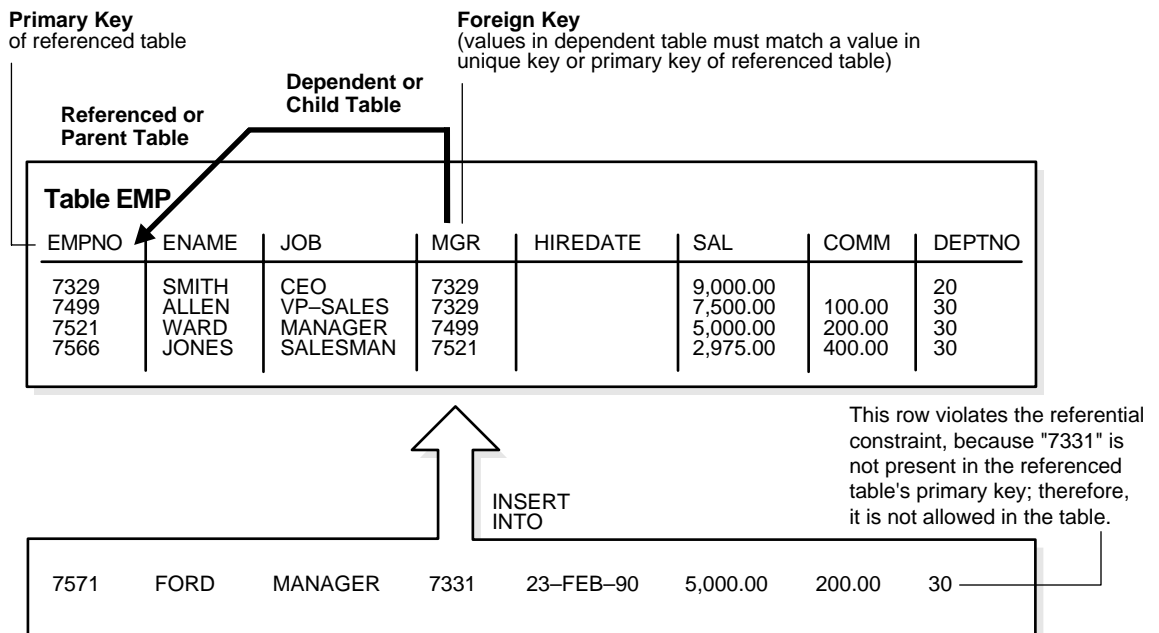
Figure 28-7 Single Table Referential Constraints
