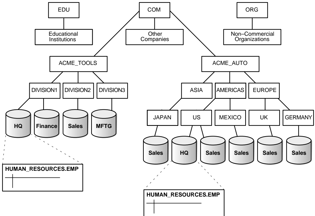
Figure 33–2 Network Directories and Global Database Names
