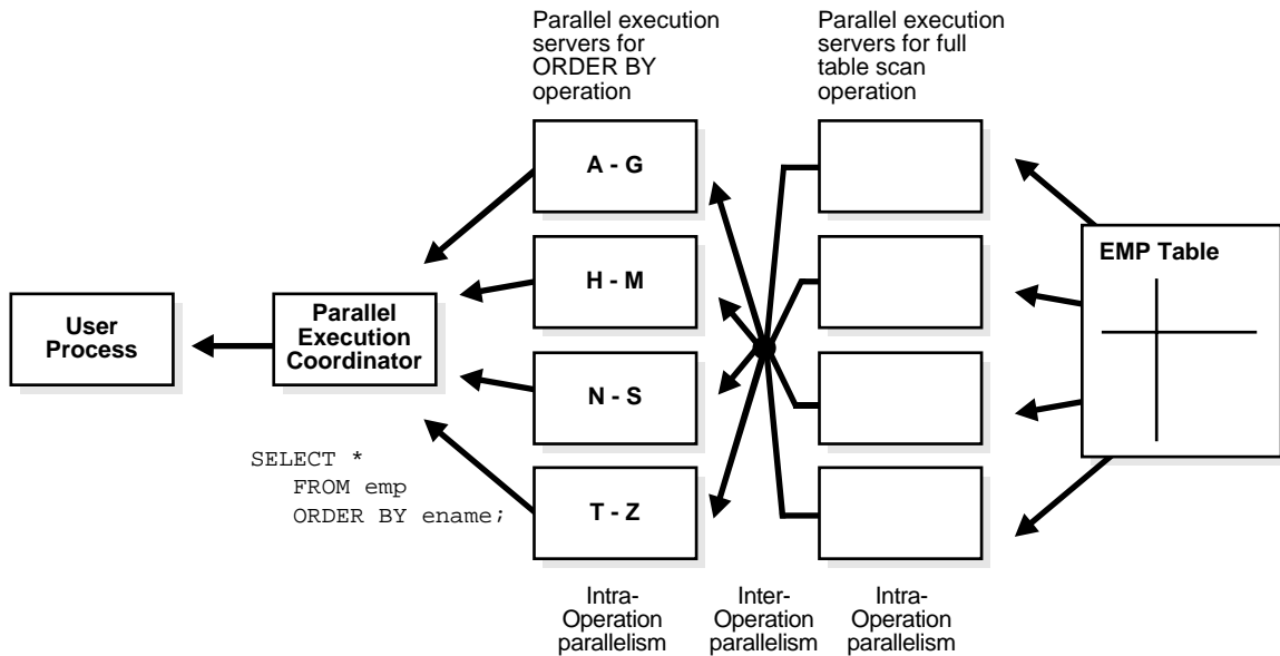
Figure 26–5 Inter-Operation Parallelism and Dynamic Partitioning
