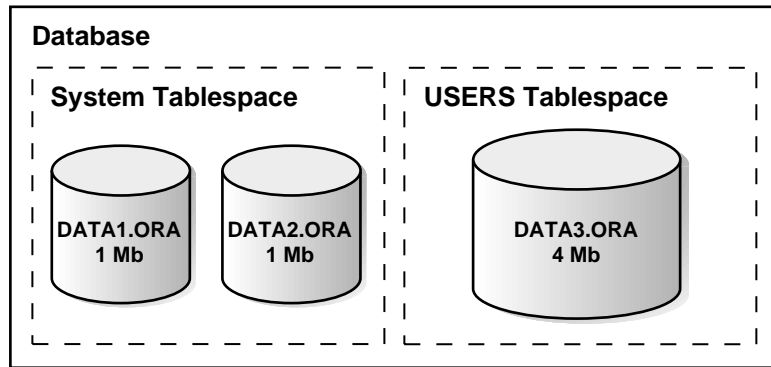
Figure 1-2 Databases, Tablespaces, and Datafiles
