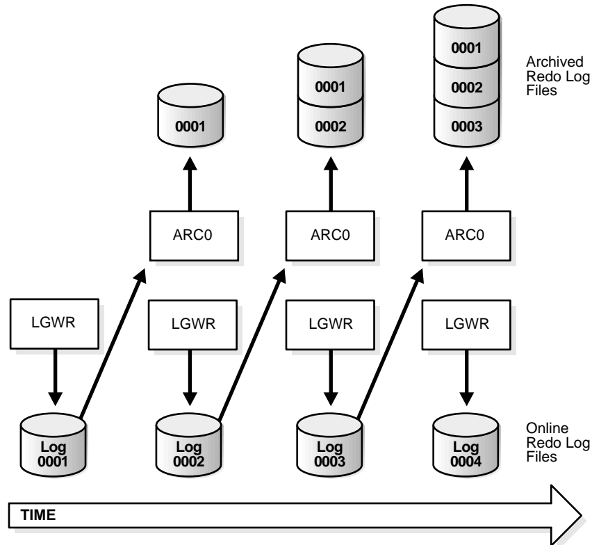
Figure 32–3 Online Redo Log File Use in ARCHIVELOG Mode
