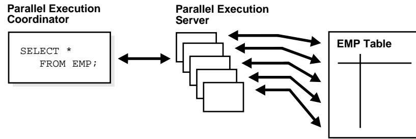
Figure 26–2 Parallel Full Table Scan
