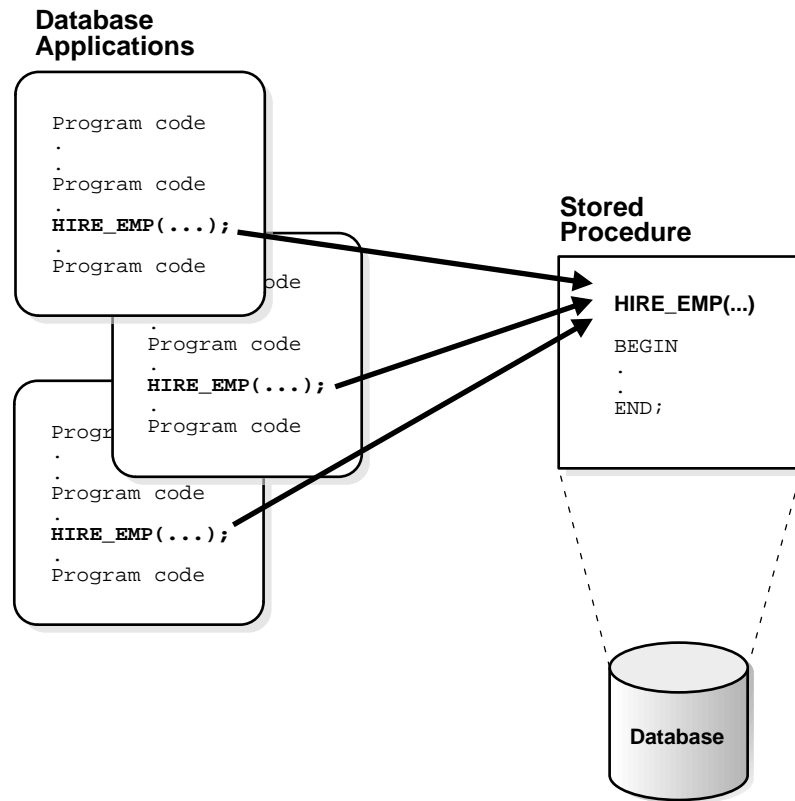
Figure 18–1 A Stored Procedure
