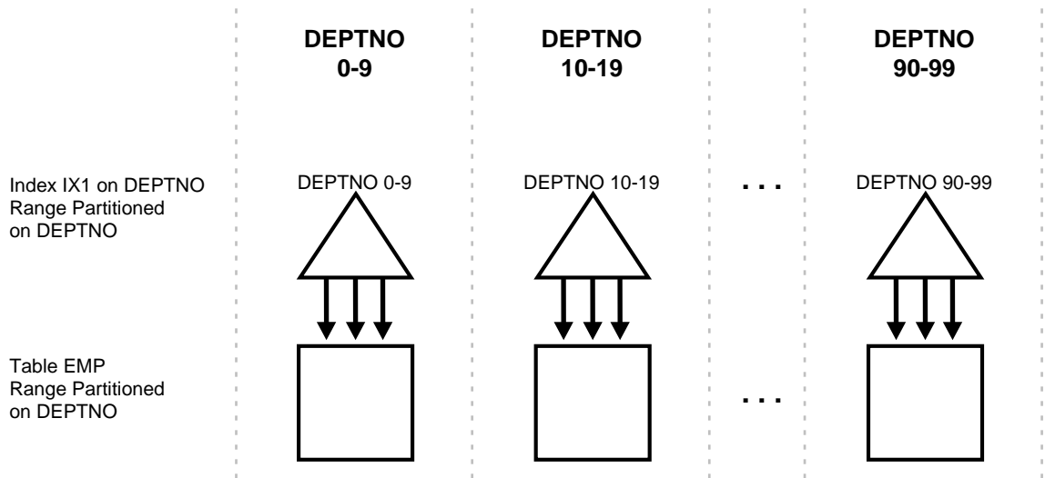
Figure 11-4 Local Prefixed Index
