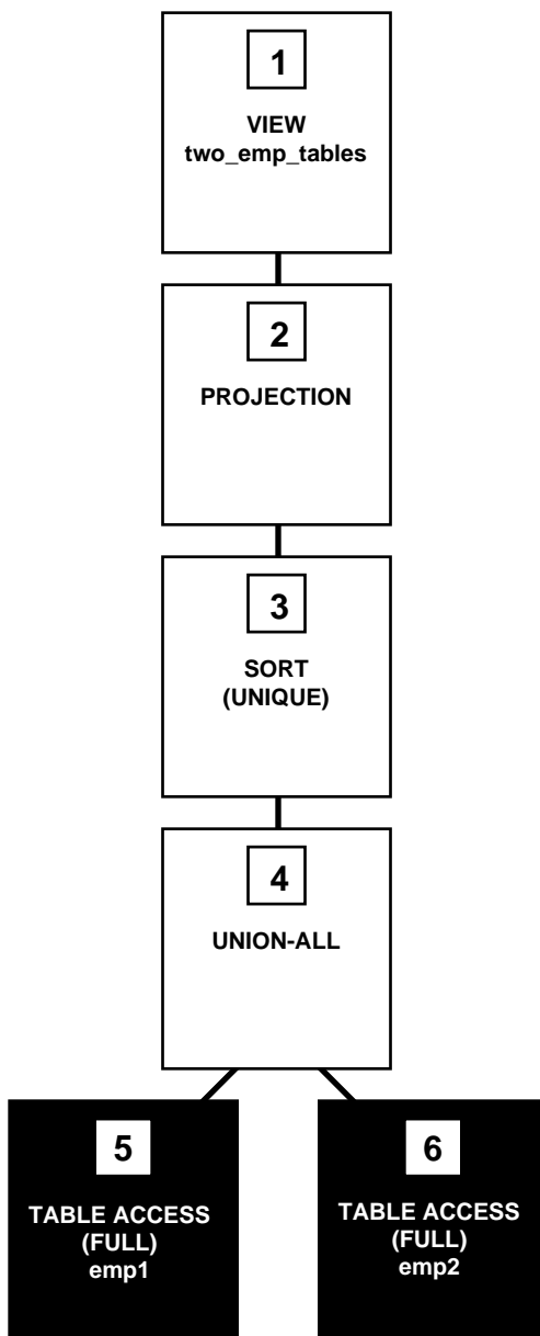
Figure 23–3 Accessing a View Defined with the UNION Set Operator
