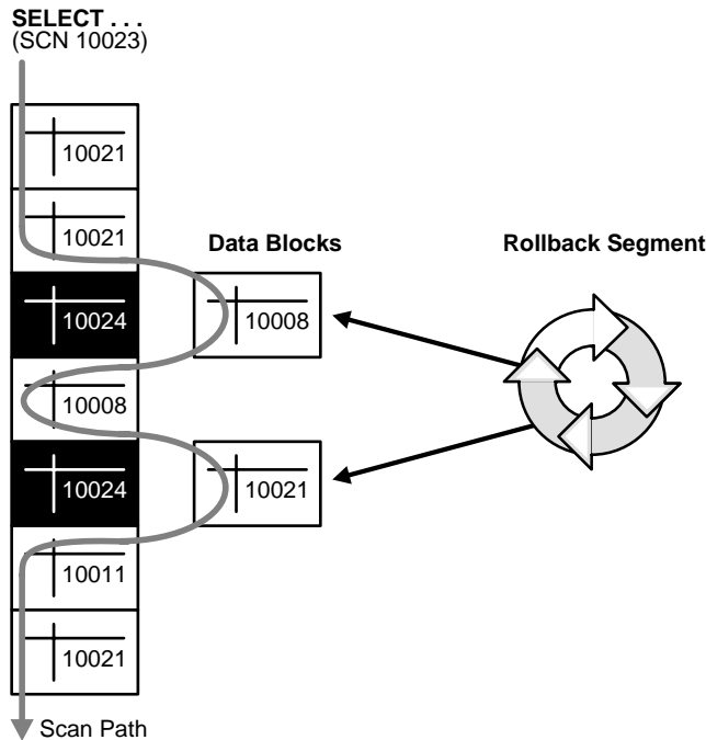
Figure 27-1 Transactions and Read Consistency
