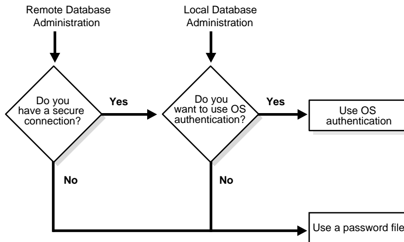
Figure 29-3 Database Administrator Authentication Methods
