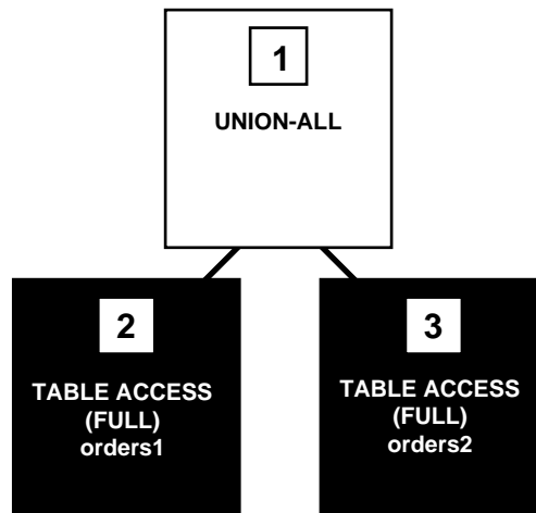
Figure 23–7 Compound Query with UNION ALL Set Operator
