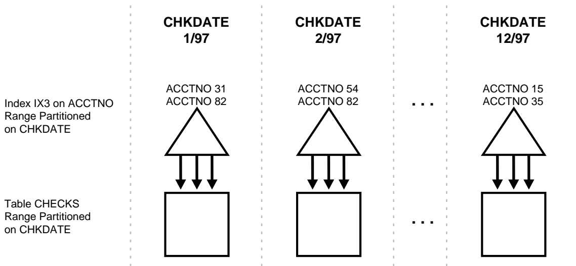
Figure 11–5 Local Nonprefixed Index
