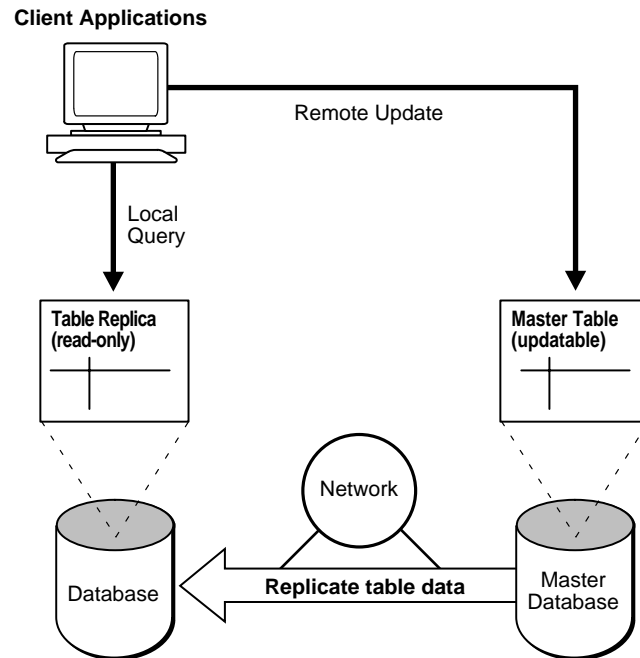
Figure 34–6 Read-Only Snapshot Replication
