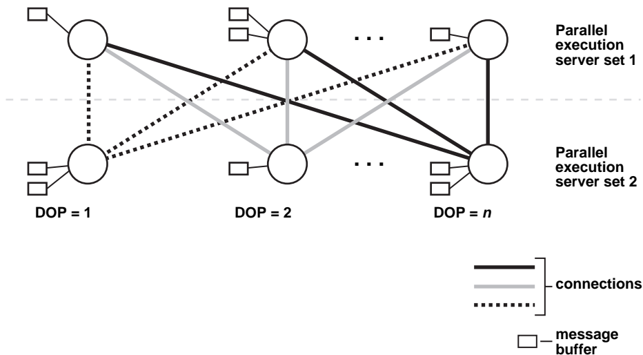
Figure 26–3 Parallel Execution Server Connections and Buffers
