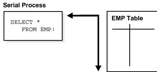
Figure 26–1 Serial Full Table Scan
