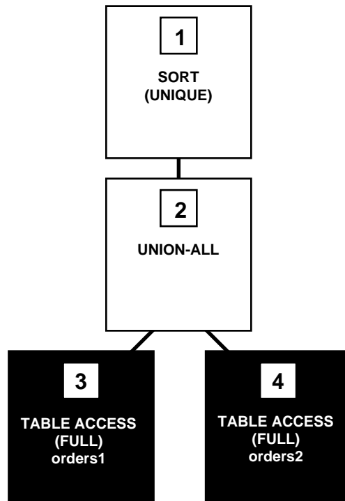
Figure 23–8 Compound Query with UNION Set Operator
