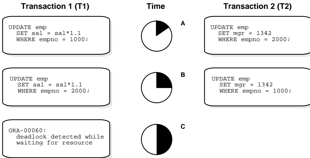
Figure 27-3 Two Transactions in a Deadlock
