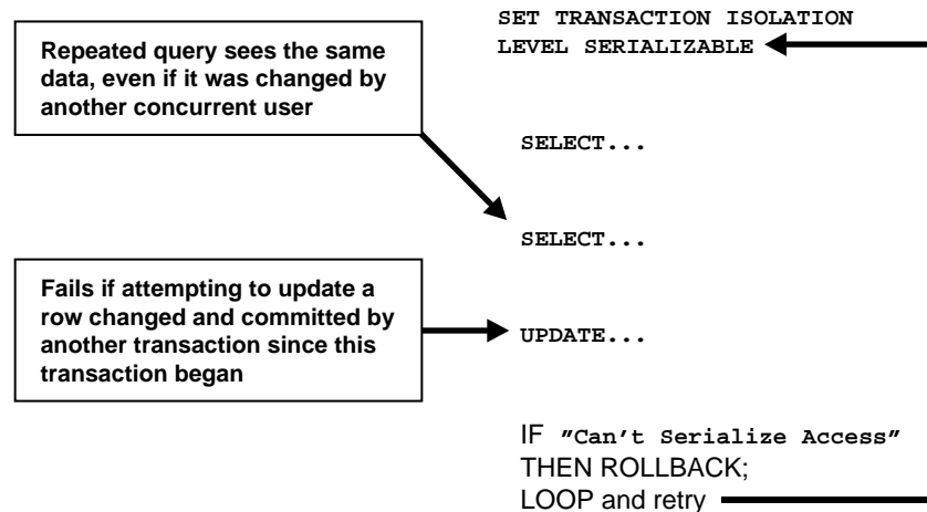
Figure 27-2 Serializable Transaction Failure
