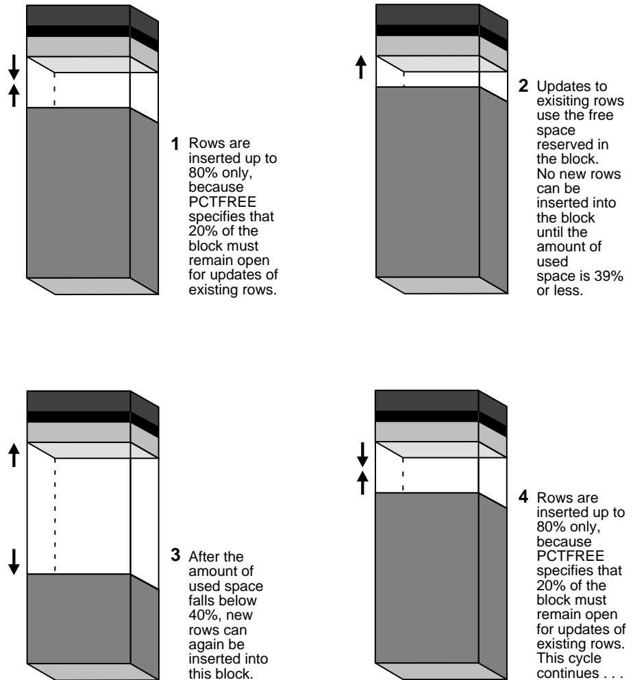
Figure 4-5 Maintaining the Free Space of Data Blocks with PCTFREE and PCTUSED
