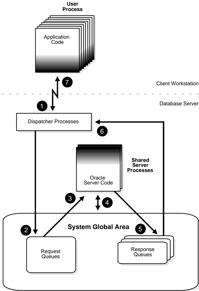
Figure 8-3 The Multi-Threaded Server Configuration and Shared Server Processes
