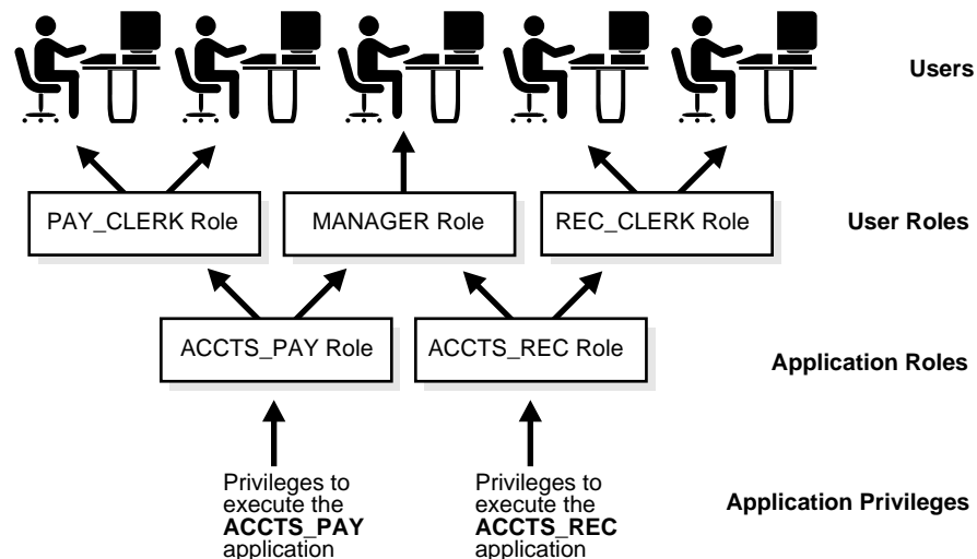
Figure 30-1 Common Uses for Roles
