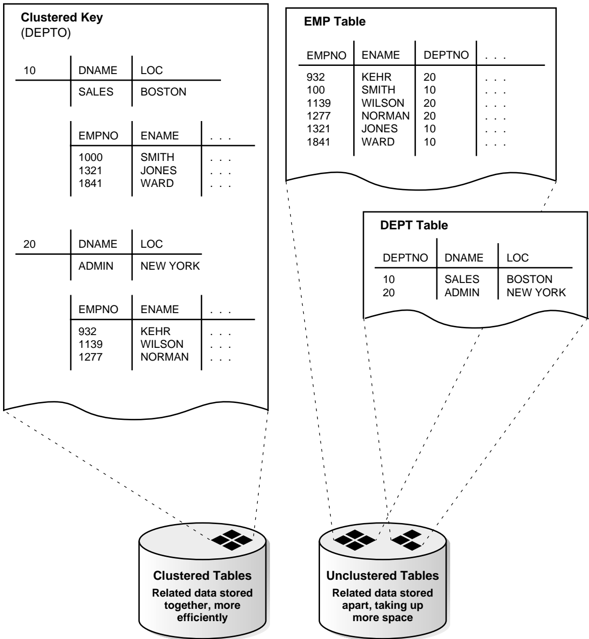
Figure 1-4 Clustered and Non-clustered Tables
