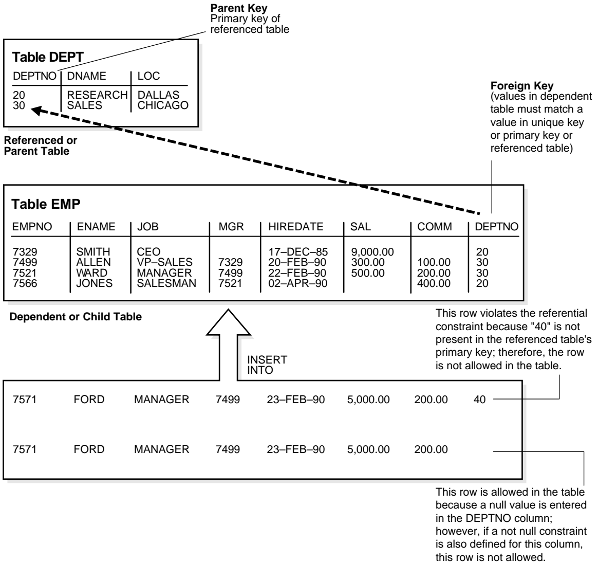
Figure 28–6 Referential Integrity Constraints
