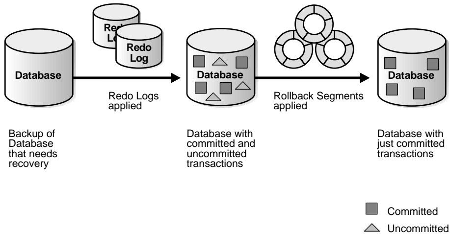
Figure 32–1 Basic Recovery Steps: Rolling Forward and Rolling Back
