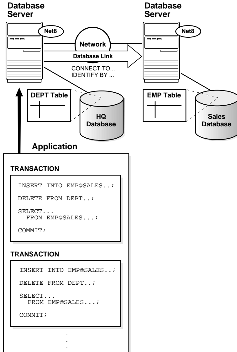
Figure 33-1 An Oracle Distributed Database System
