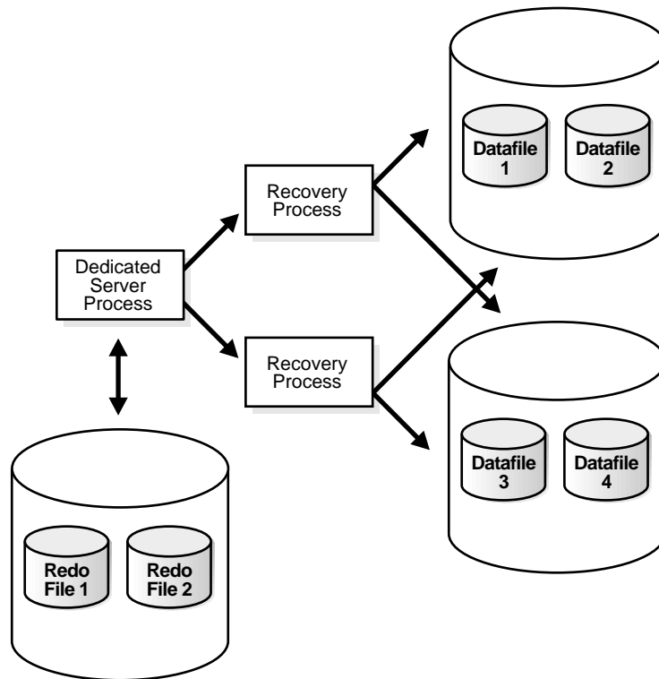
Figure 32-2 Typical Parallel Recovery Session
