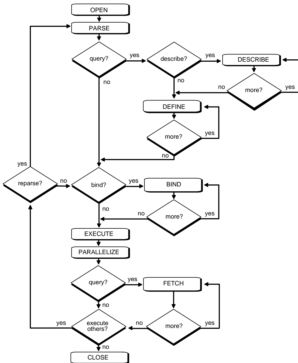
Figure 16-1 The Stages in Processing a SQL Statement
