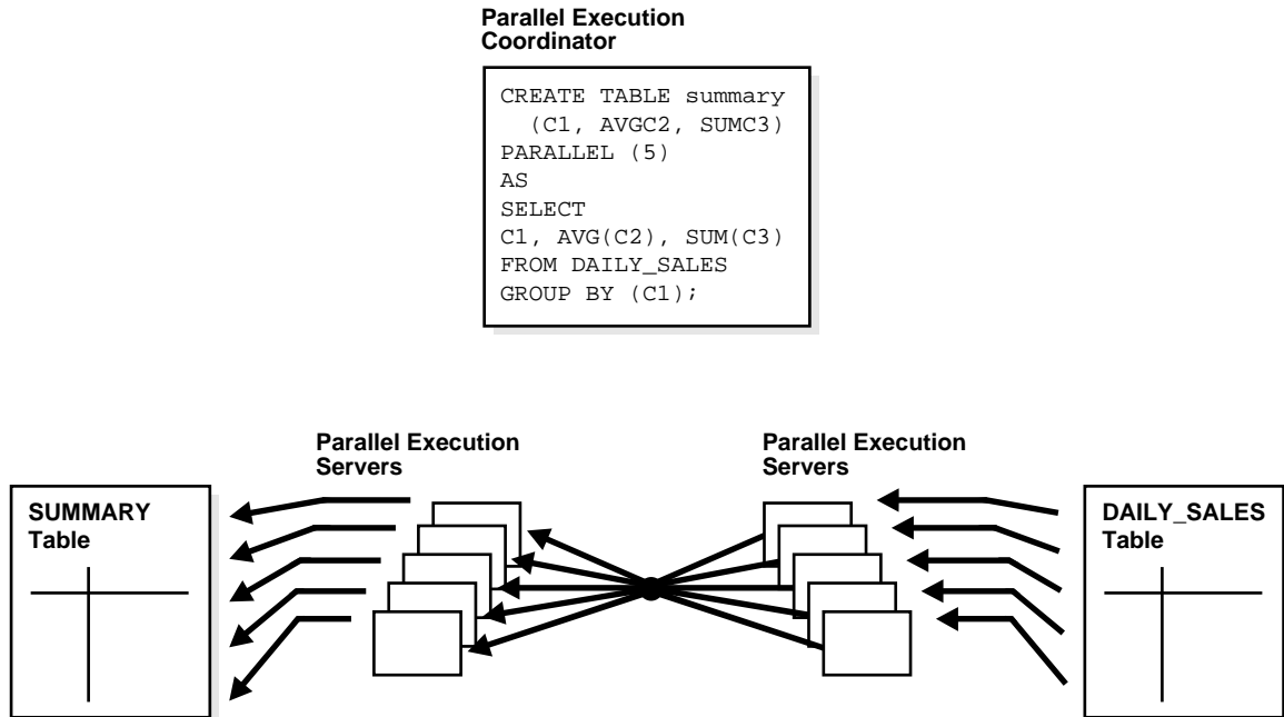
Figure 26–6 Creating a Summary Table in Parallel
