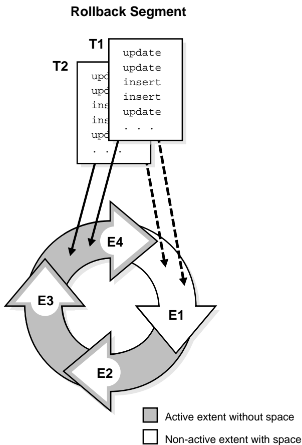
Figure 4–7 Cyclical Use of the Allocated Extents in a Rollback Segment
