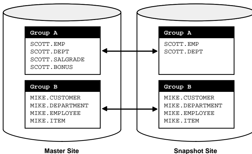
Figure 34–2 Snapshot Groups Correspond with Master Groups
