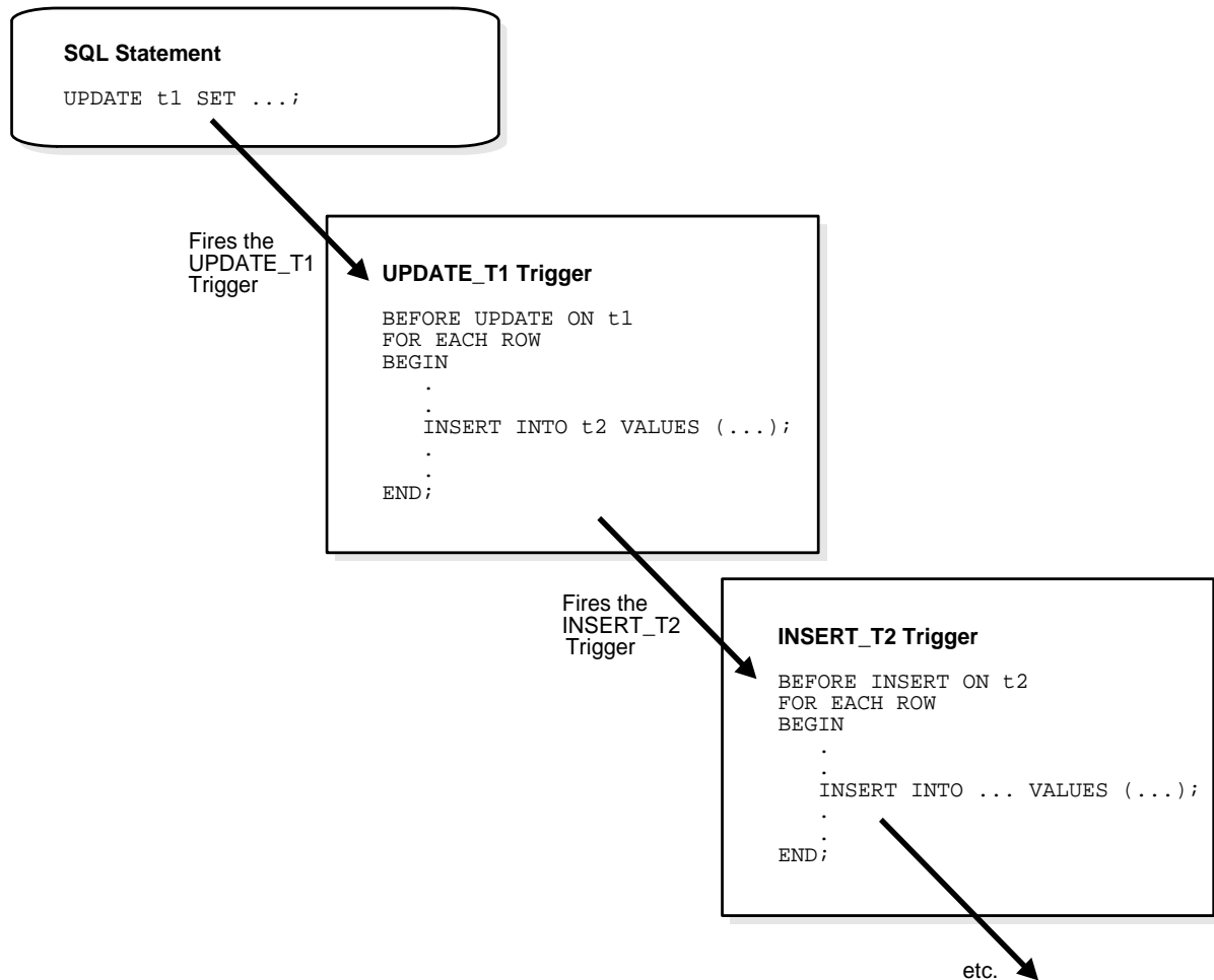
Figure 20–2 Cascading Triggers
