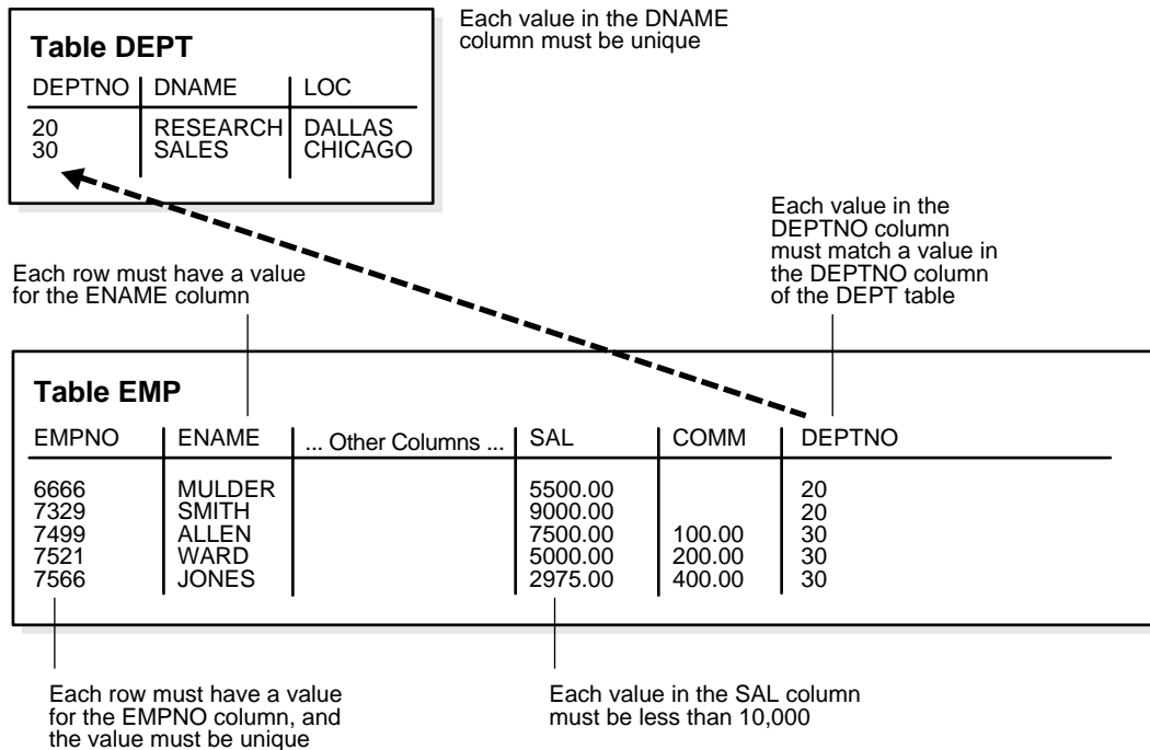
Figure 28-1 Examples of Data Integrity
