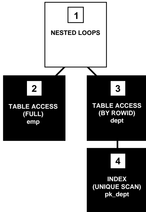
Figure 24-1 Nested Loops Join
