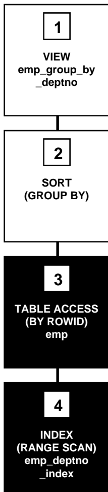
Figure 23-4 Accessing a View Defined with a GROUP BY Clause
