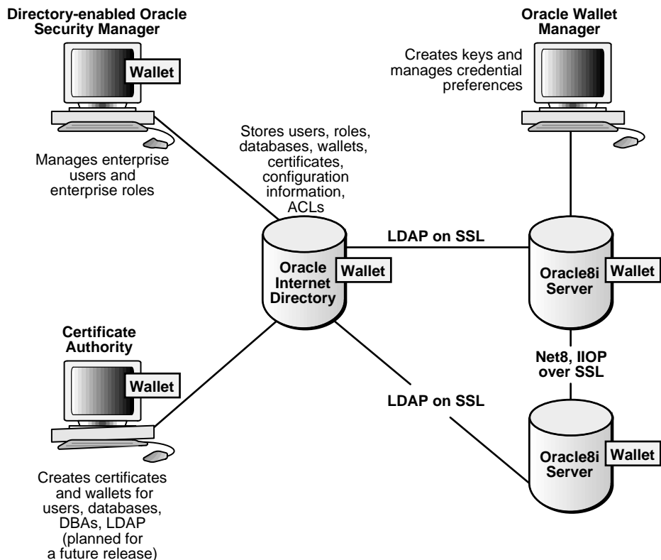
Figure 29–1 Oracle Public Key Infrastructure
