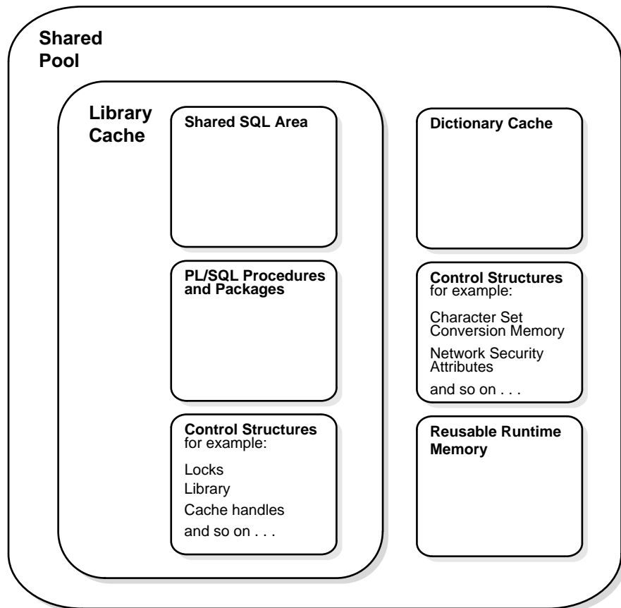
Figure 7–1 Contents of the Shared Pool
