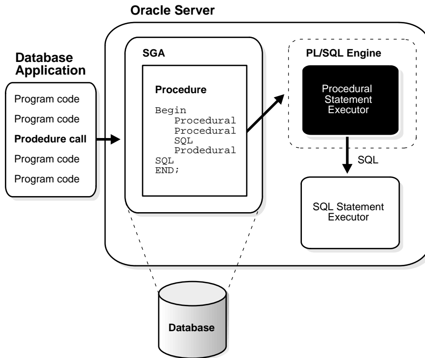
Figure 16–2 The PL/SQL Engine and the Oracle Server
