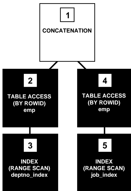
Figure 23-1 Execution Plan for a Transformed Query Containing OR
