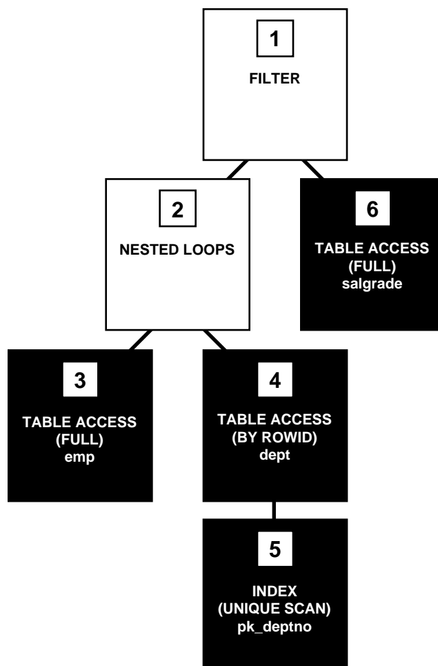
Figure 22–1 An Execution Plan
