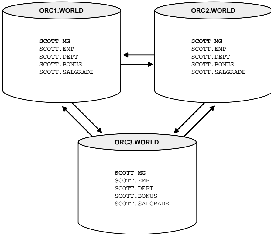
Figure 34–1 Master Group SCOTT_MG contains same replication objects at all sites.
