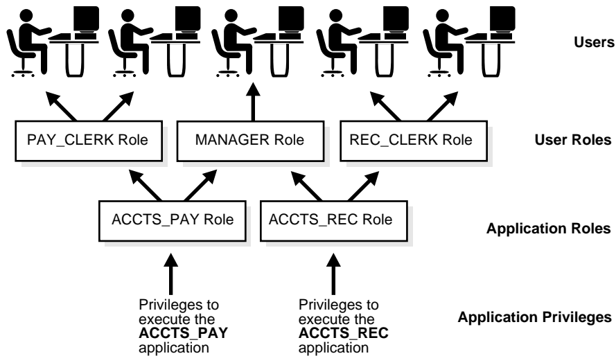
Figure 1–5 Oracle Security Features
