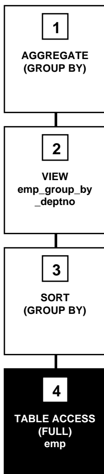
Figure 23–5 Applying Aggregate Functions to a View Defined with GROUP BY Clause
