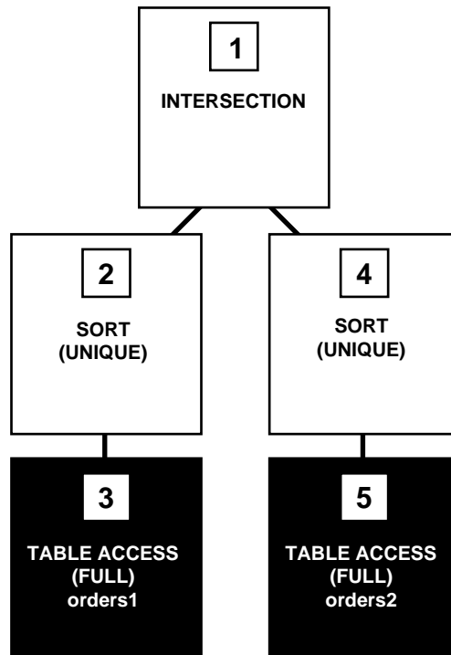
Figure 23-9 Compound Query with INTERSECT Set Operator
