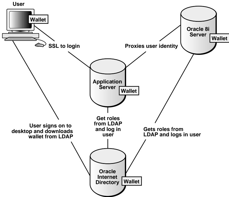
Figure 29–2 Multi-Tier Authentication
