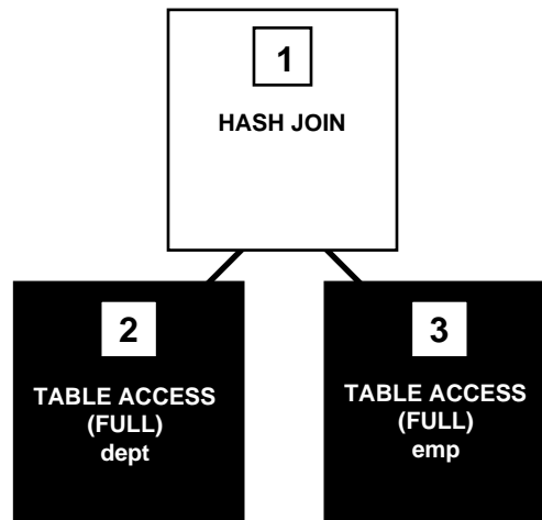
Figure 24-4 Hash Join
