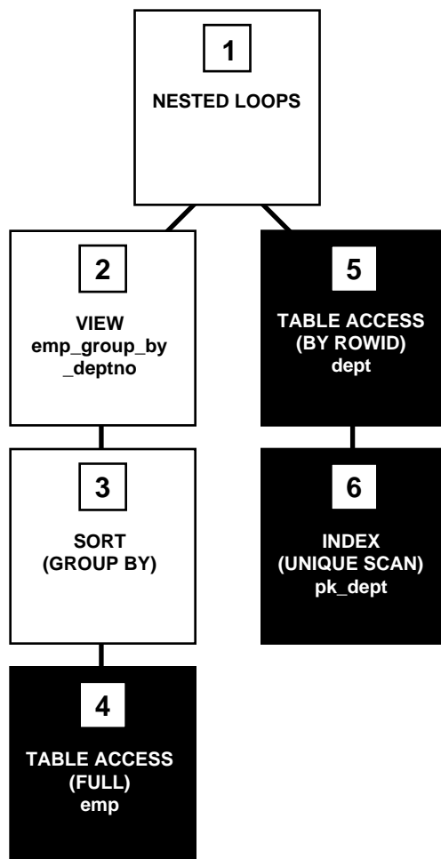
Figure 23–6 Joining a View Defined with a GROUP BY Clause to a Table
